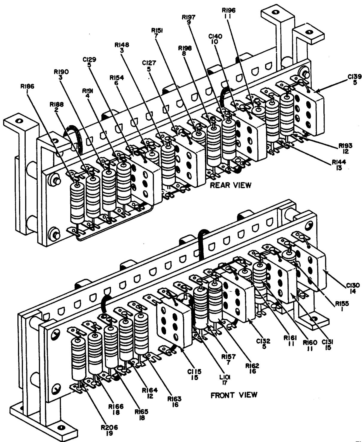
Figure 11. Generator, Signal TS-621A/U, TS-621B/U, SG-557/U, Board Assembly, Resistor "C"
