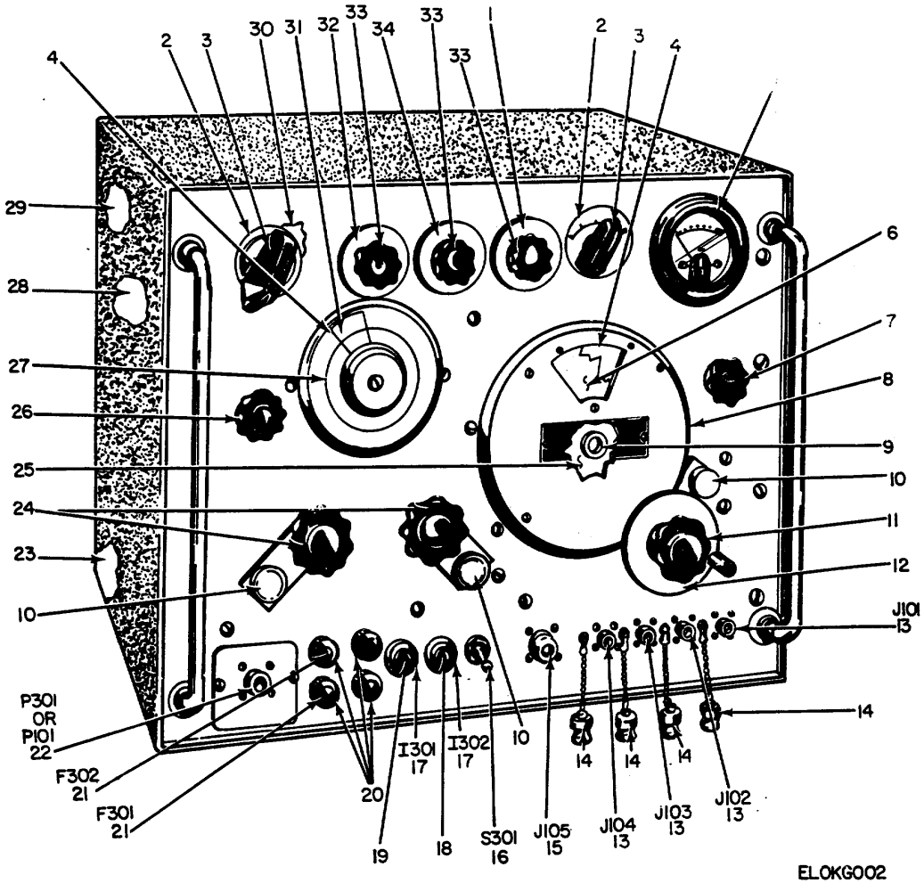
Figure 2. Generator, Signal TS-621A/U, TS-621B/U, SG-557/U.
