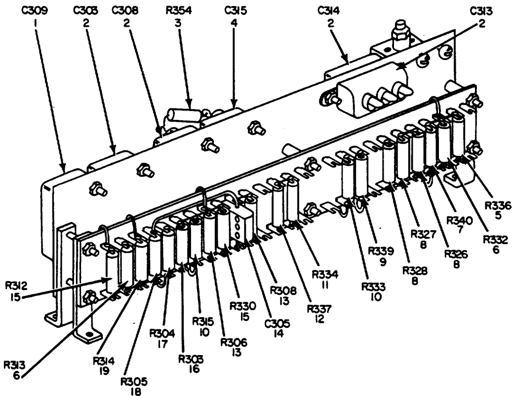
Figure 16. Generator, Signal TS-621A/U, TS-621B/U, SG-557/U, Board Assembly, Resistor "F".
