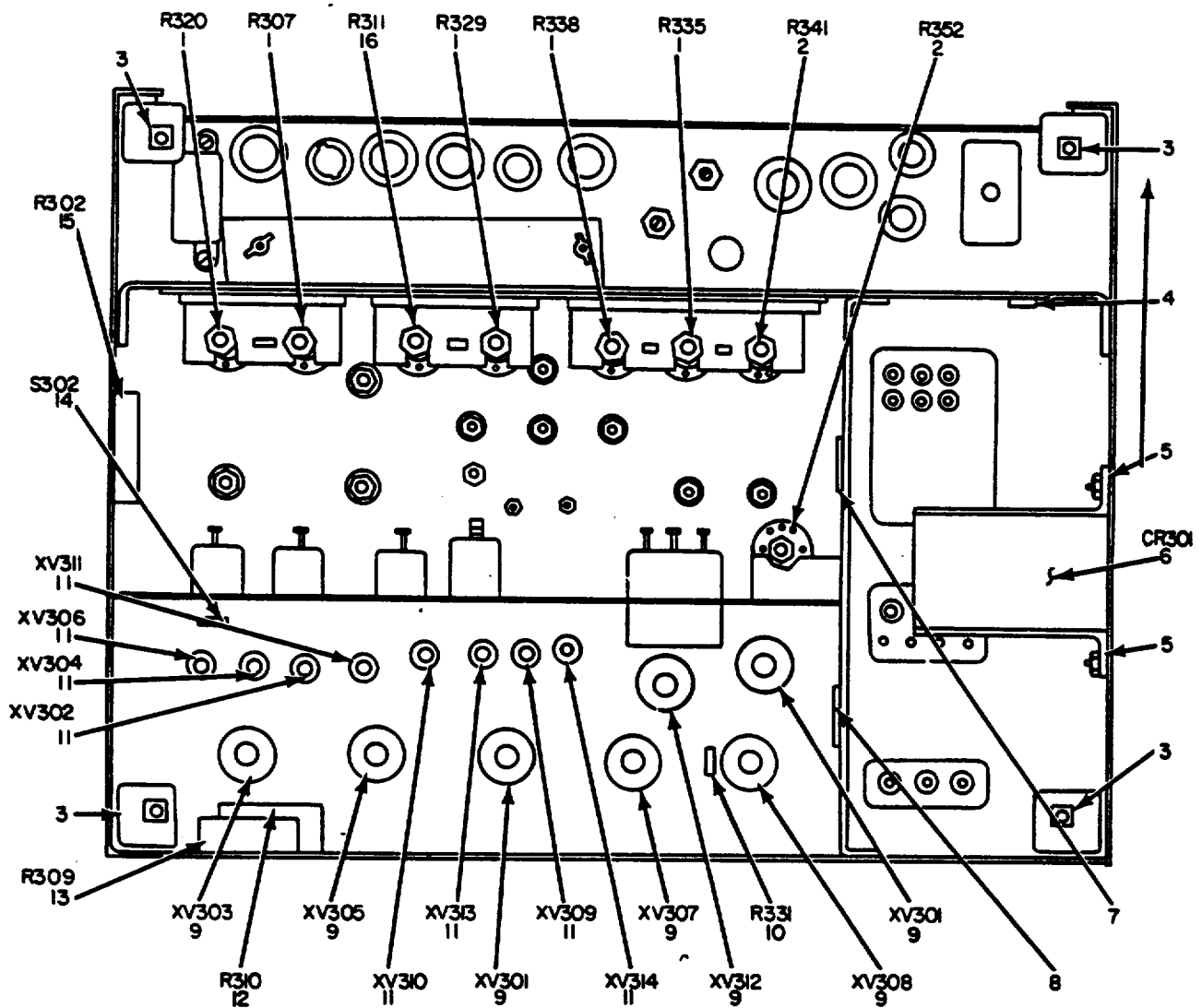
Figure 13. Generator, Signal TS-621A/U, TS-621B/U, SG-557/U, Deck Assembly, Power, Front Panel Removed.
