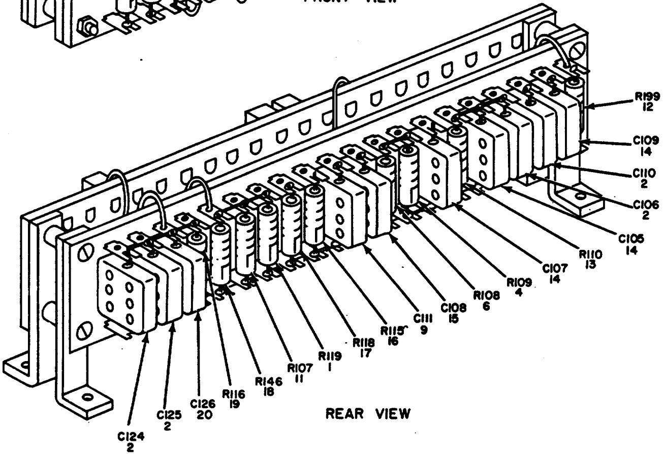
Figure 12. Generator, Signal TS-621A/U, TS-621B/U, SG-557/U, Board Assembly, Resistor "D".
