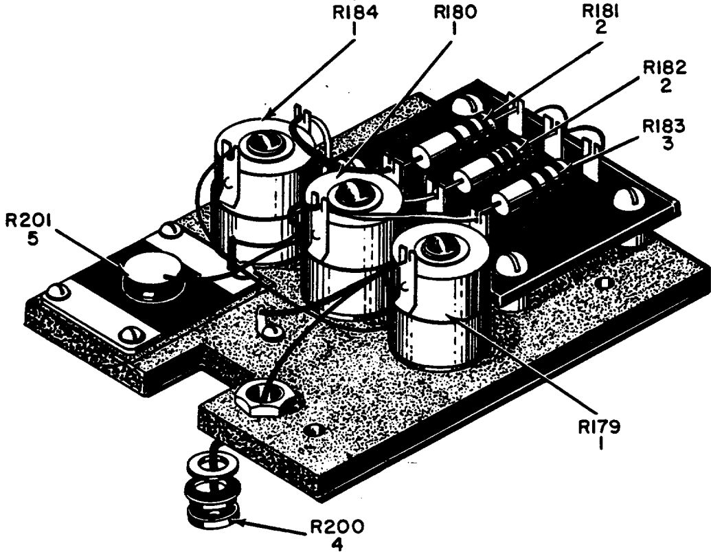
Figure 7. Generator, Signal TS-621A/U, TS-621B/U, SG-557/U, Board Assembly, Resistor "H".
