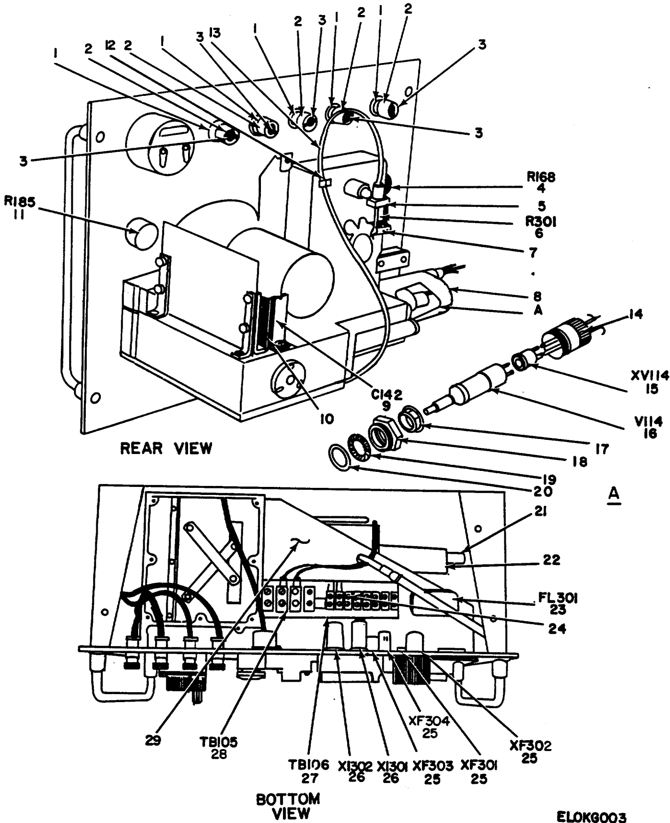
Figure 3. Generator, Signal TS-621A/U, TS-621B/U, SG-557/U, Panel Assembly.
