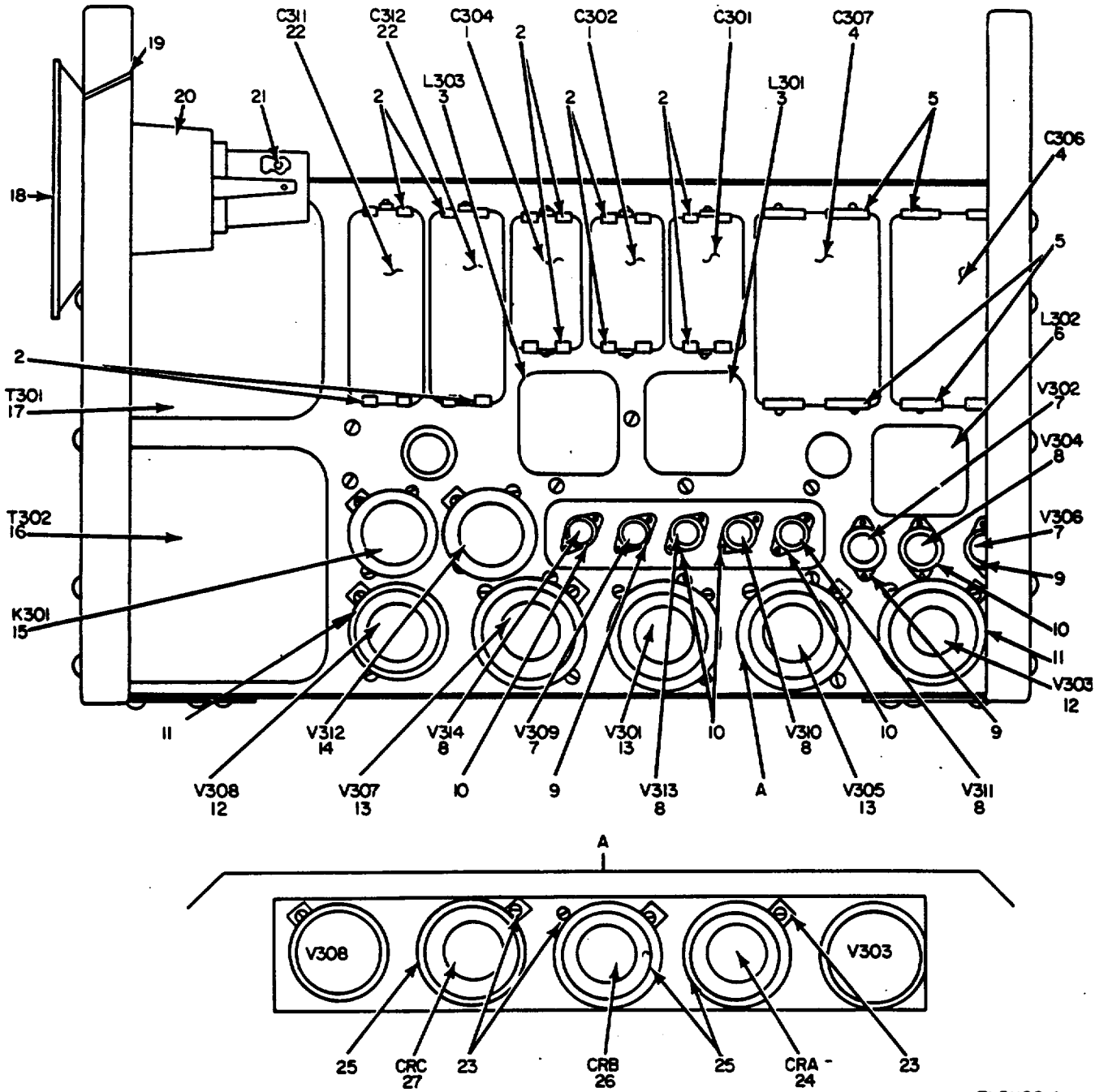
Figure 14. Generator, Signal TS-621A/U, TS-621B/U, SG-557/U, Deck Assembly, Power, Top View.
